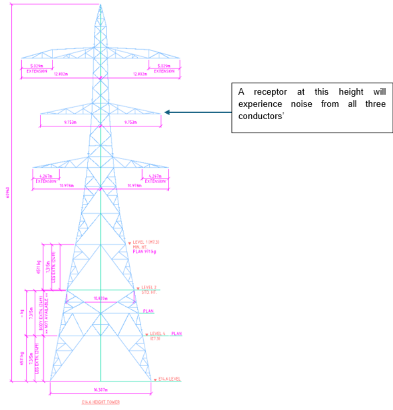
Figure 8.1: Elevation of ZBC44 Transmission Pylon
