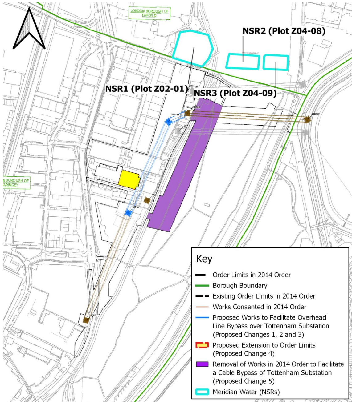
Figure 6.1 Extract from Concept Plan and annotated with NSRs
